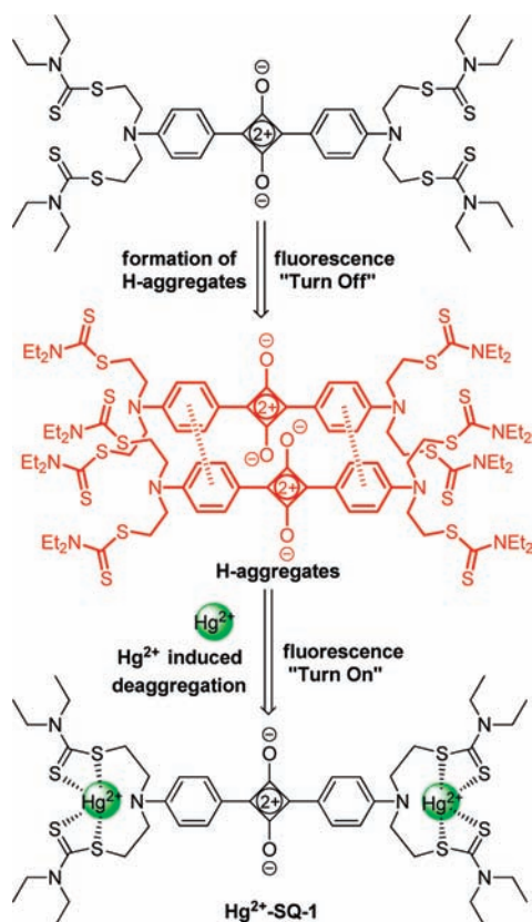
Figure 5. Process of sensing Hg 2+ and the proposed binding model of “Hg 2+ -SQ-1”.
