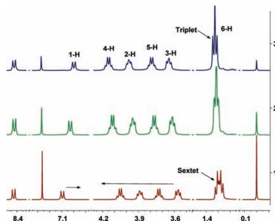
Figure 4. ^1\text{H} NMR spectrum of SQ-1 in \text{CDCl}_3 with increasing concentration of (\text{CH}_3\text{COO})_2\text{Hg} . The mole ratio of [(\text{CH}_3\text{COO})_2\text{Hg}] to [\text{SQ-1}] is (1) 0, (2) 1.0, and (3) 2.2, respectively.
