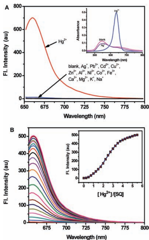
Figure 3. (A) Fluorescence spectrum of SQ-1 ( 2\ \mu\text{M} ) in the presence of different metal ions (5 equiv) in AcOH– \text{H}_2\text{O} (40:60, v/v) solution. Inset: The corresponding absorption spectrum of SQ-1 and in the presence of \text{Ag}^+ or \text{Hg}^{2+} . (B) Change in fluorescence intensity of SQ-1 ( 2\ \mu\text{M} ) with increasing addition of \text{Hg}^{2+} (0– 11\ \mu\text{M} ) in AcOH– \text{H}_2\text{O} (40:60, v/v) solution. Inset: The binding isotherm of SQ-1 at 660 nm upon the addition of \text{Hg}^{2+} . Error bars for n = 3 ( \lambda_{\text{ex}} = 644\ \text{nm} , slit: 5 nm/5 nm, PMT Volts: 600).
